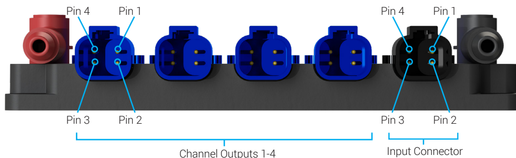
Mating connector (AT06-4S Blue)
